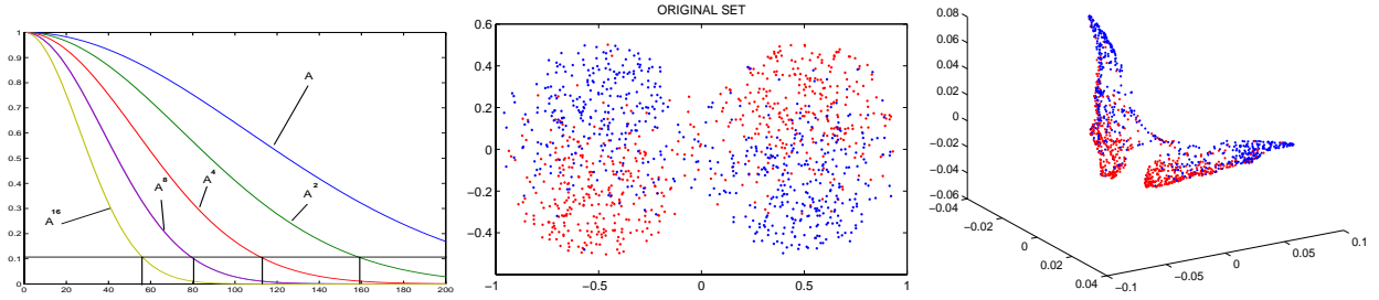
FIGURE 1. Left: spectra of some powers of A . Middle and right: consider a mixture of two materials with different heat conductivity. The original geometry (middle) is mapped as a “butterfly” set, in which the red (higher conductivity) and blue phases are organized according to the diffusion they generate: the cord length between two points in the diffusion space measures the quantity of heat that can travel between these points.
